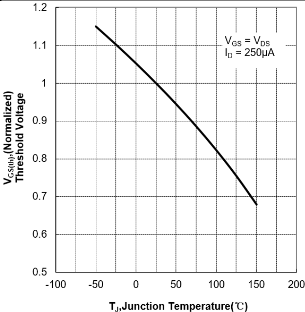
Figure 8 Typical Threshold Voltage vs Junction Temperature
