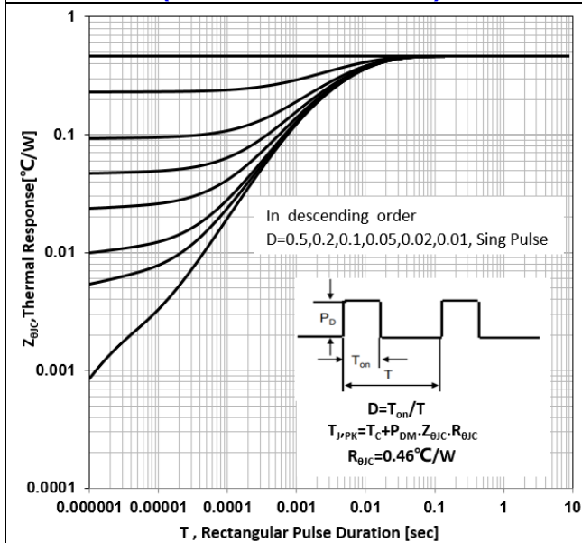
Figure 3a Max Thermal Impedance (TO-220/TO-3PN/TO-247)
