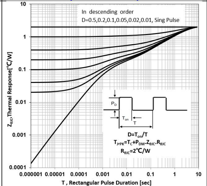
Figure 3b Max Thermal Impedance (TO-220F/TO-3PF)
