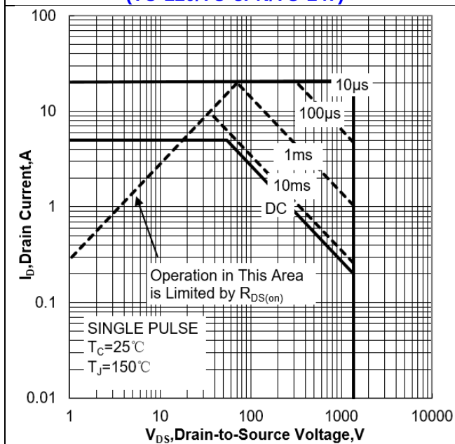
Figure 1a Safe Operating Area (TO-220/TO-3PN/TO-247)
