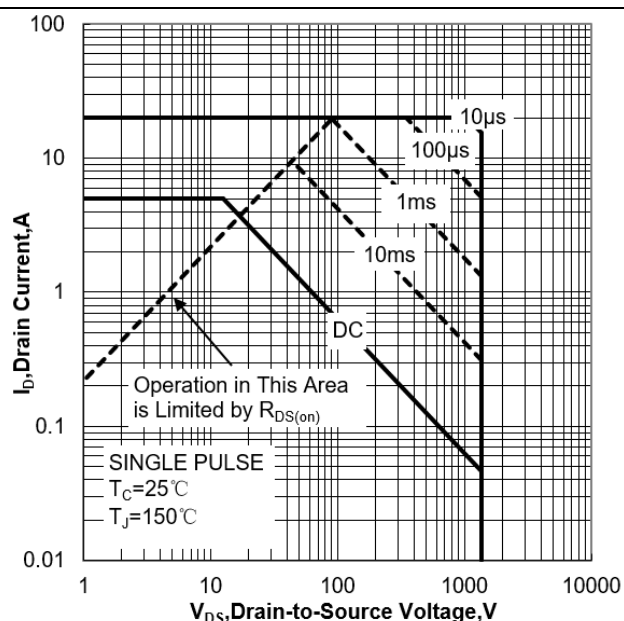
Figure 1b Safe Operating Area (TO-220F/TO-3PF)
