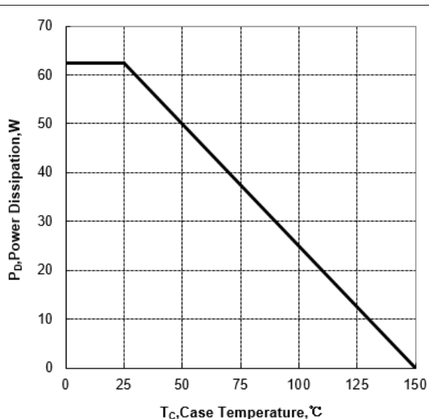
Figure 2b Power Dissipation (TO-220F/TO-3PF)
