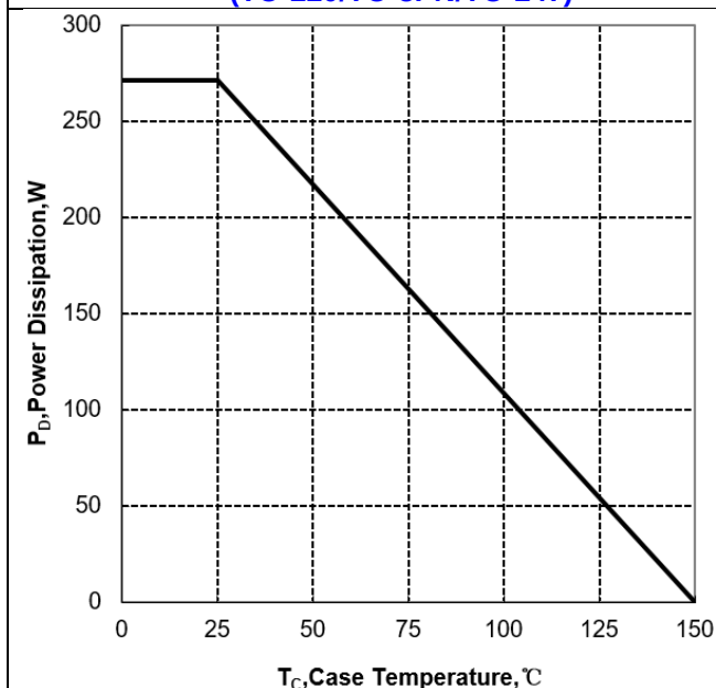
Figure 2a Power Dissipation (TO-220/TO-3PN/TO-247)
